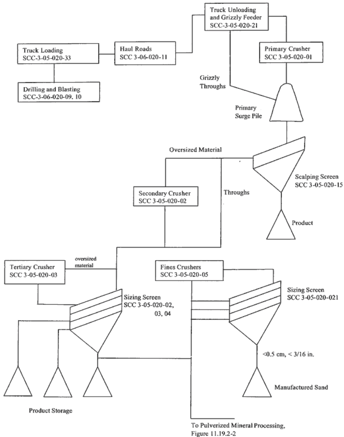
Figure 11.19.2-1. Typical stone processing plant
